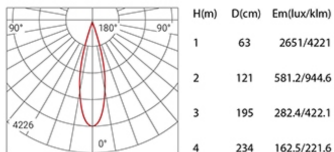
Beam Angle 24° 25W 3000K
