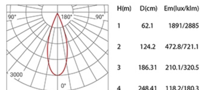
Beam Angle 38° 20W 3000K
