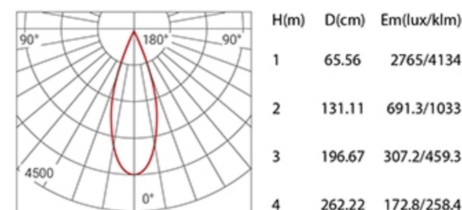
Beam Angle 38° 30W 3000K
