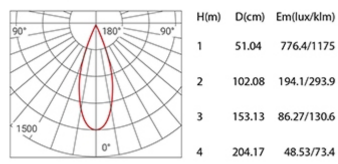
Beam Angle 38° 6W 3000K
