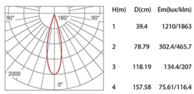
Beam Angle 24° 6W 3000K
