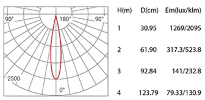
Beam Angle 15° 6W 3000K
