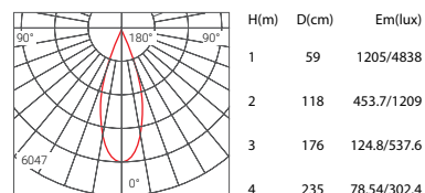
Beam Angle 38° 20W 3000K
